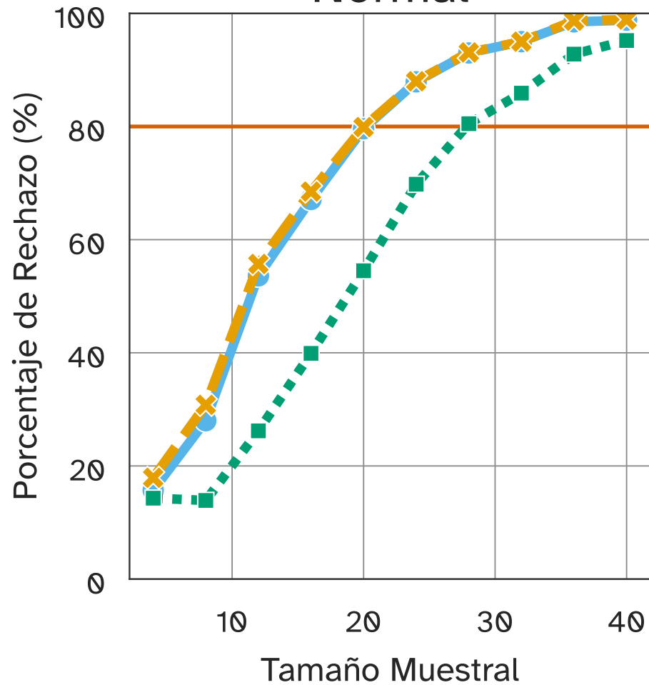
Normal
